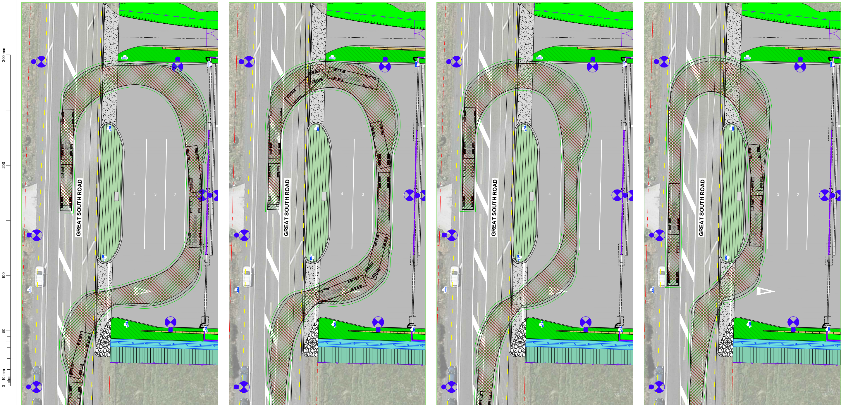
TRACKING CURVES - 23.0m TRUCK AND TRAILER SCALE: 1:250(A1), 1:500(A3)
