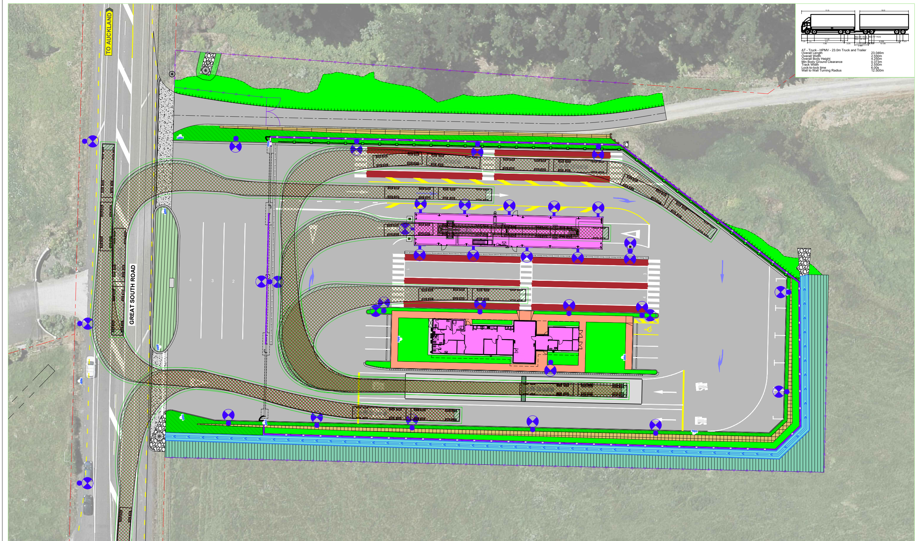
TRACKING CURVES - 23.0m TRUCK AND TRAILER SCALE: 1:250(A1), 1:500(A3)
