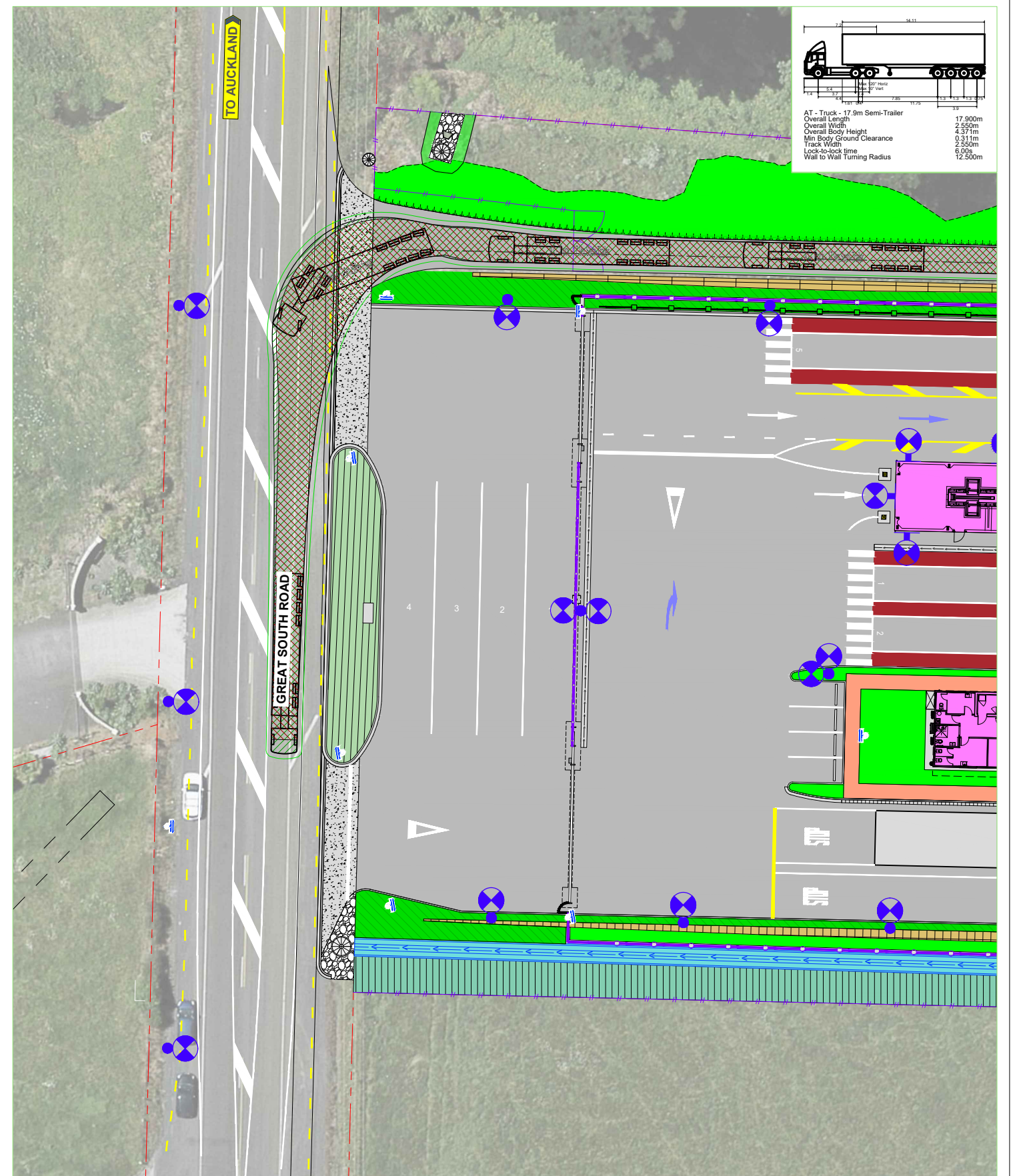
TRACKING CURVES - 17.9m SEMI-TRAILER SCALE: 1:250(A1), 1:500(A3)
