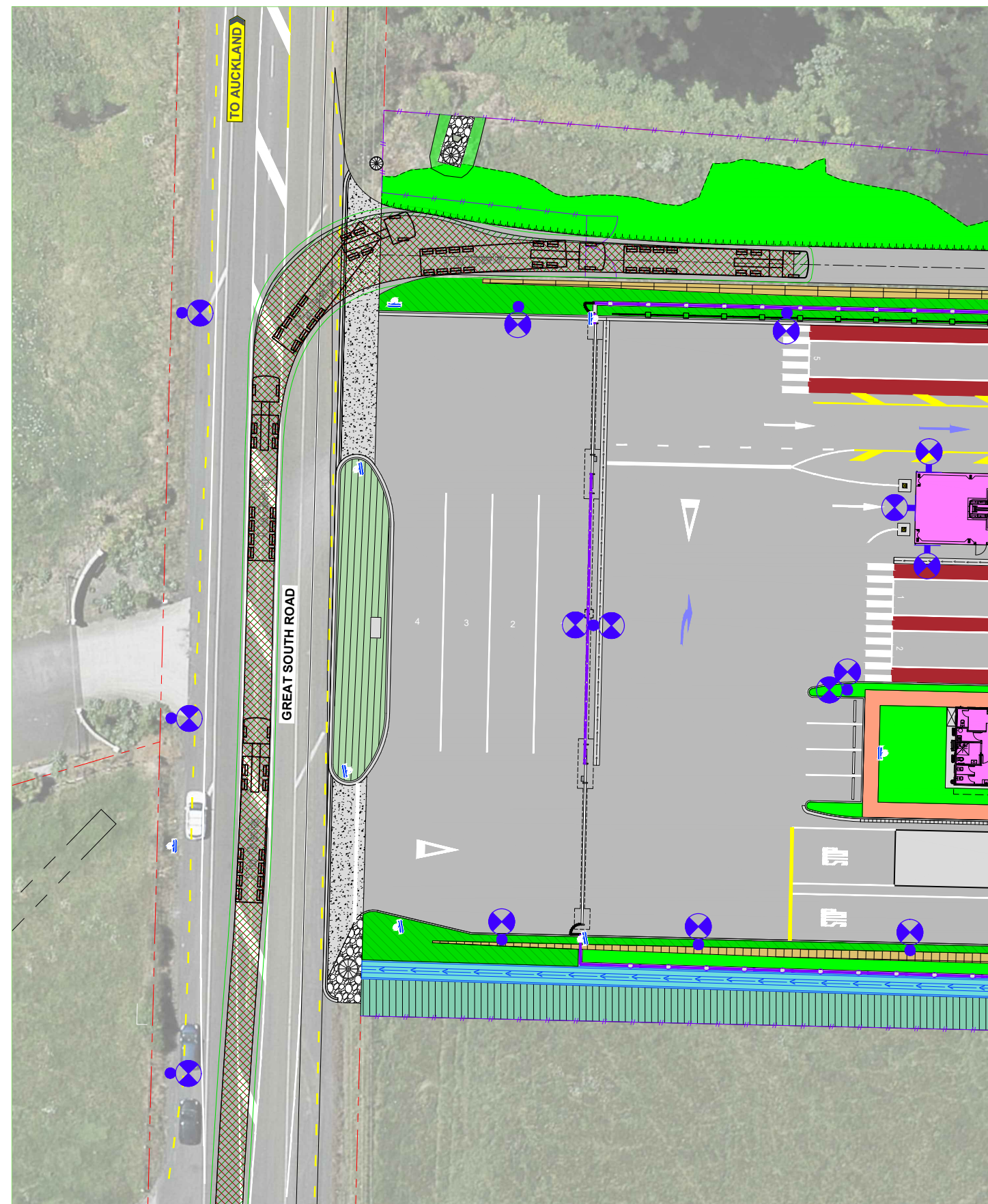
TRACKING CURVES - 17.9m SEMI-TRAILER SCALE: 1:250(A1), 1:500(A3)
